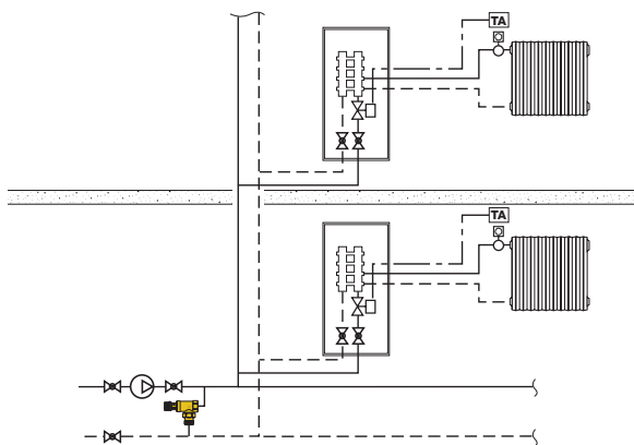
Small-medium size system, by-pass in central plant
