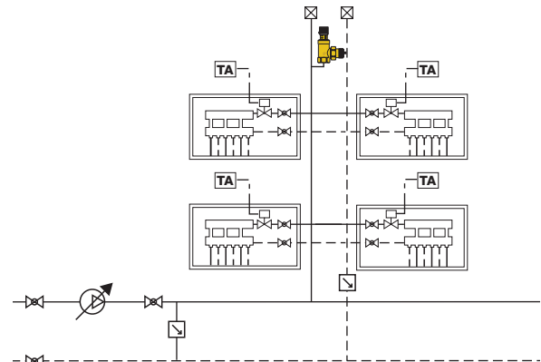
Medium-large size system, by-pass on top of risers
