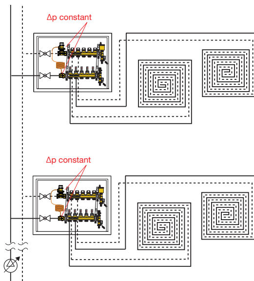
\Delta p control on manifold type systems
