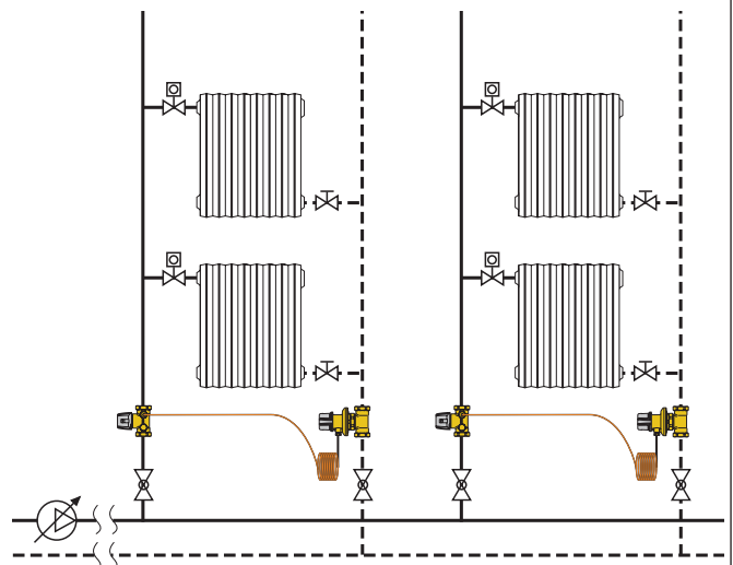
\Delta p control on riser type systems
